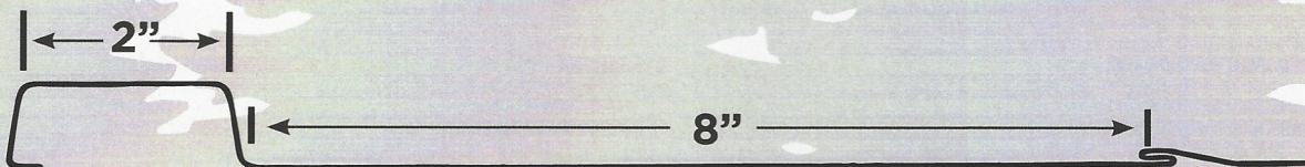
Overlap Detail
